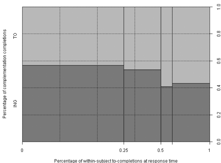
Figure 3. Spinogram of RESPONSE_CODE \times SELF_TO_RATIO
