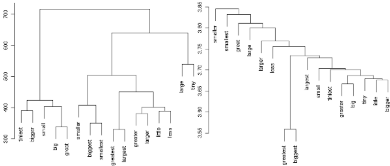
Figure 3: Dendrograms of the BP vectors with random adjective assignments
