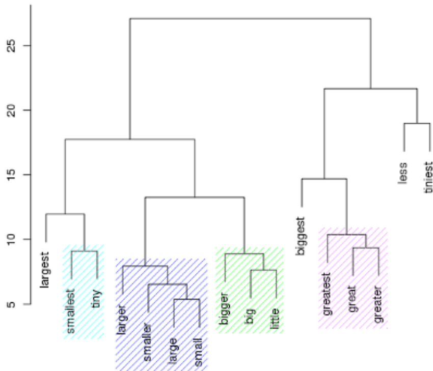
Figure 4: Dendrogram of the cluster analysis of the BP vector involving semantic ID tags
