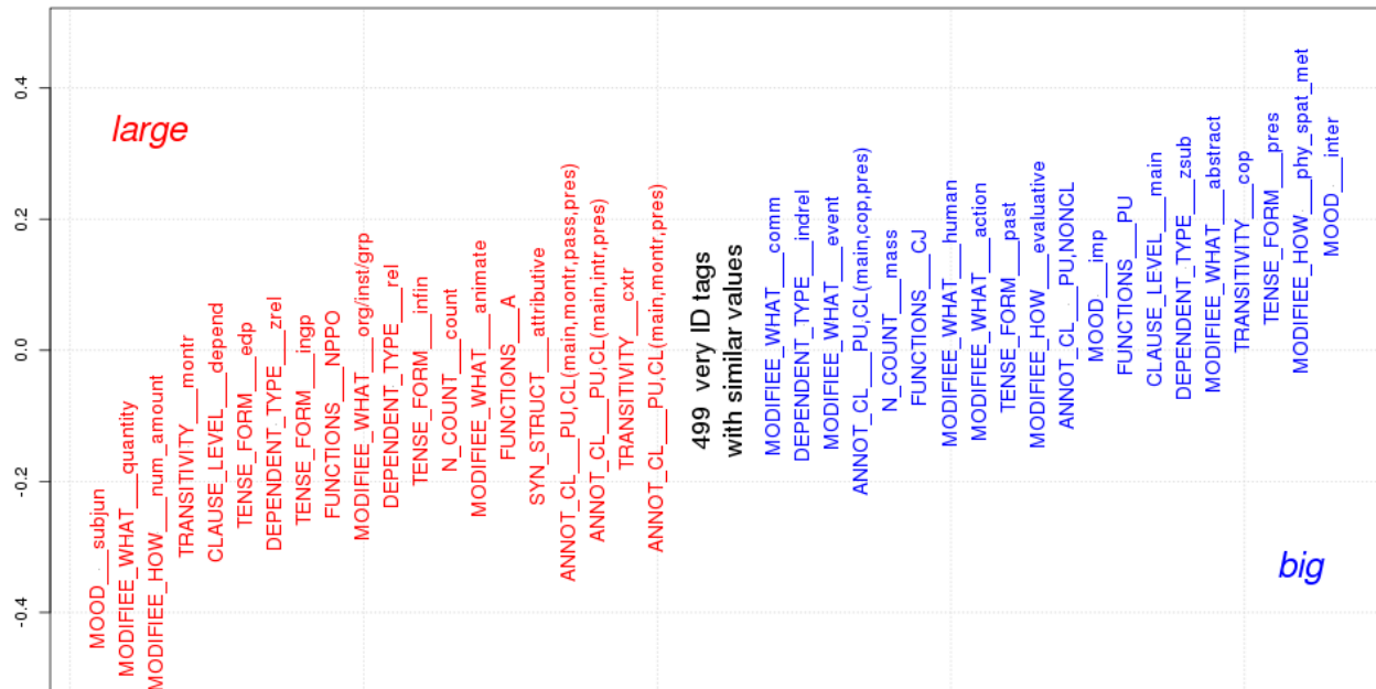
Figure 6: Snakeplot of differences between BP vector values: % big - % large
