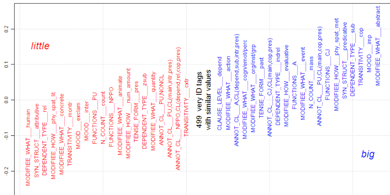
Figure 5: Snakeplot of differences between BP vector values: % big - % little
